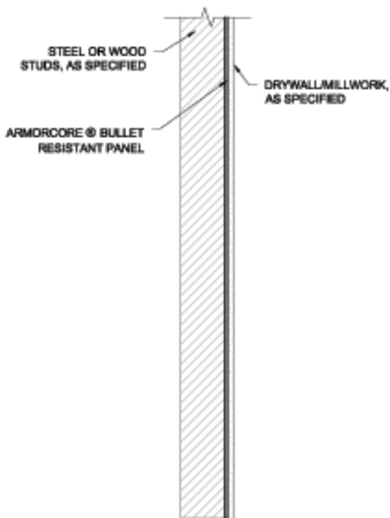
SECTION VIEW
