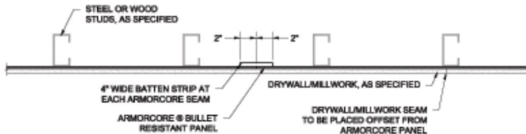
PLAN VIEW
